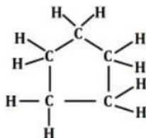
Cyclopentane
