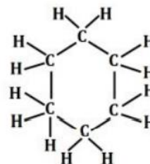
Cyclohexane
