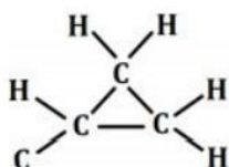
Cyclopropane
